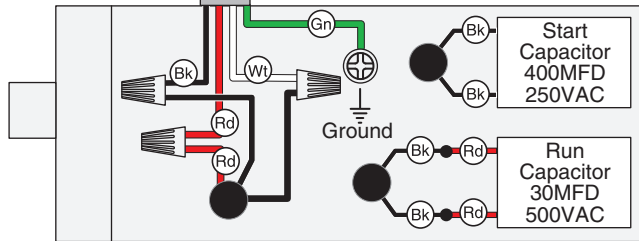
MOTOR 5HP 220V SINGLE-PHASE
